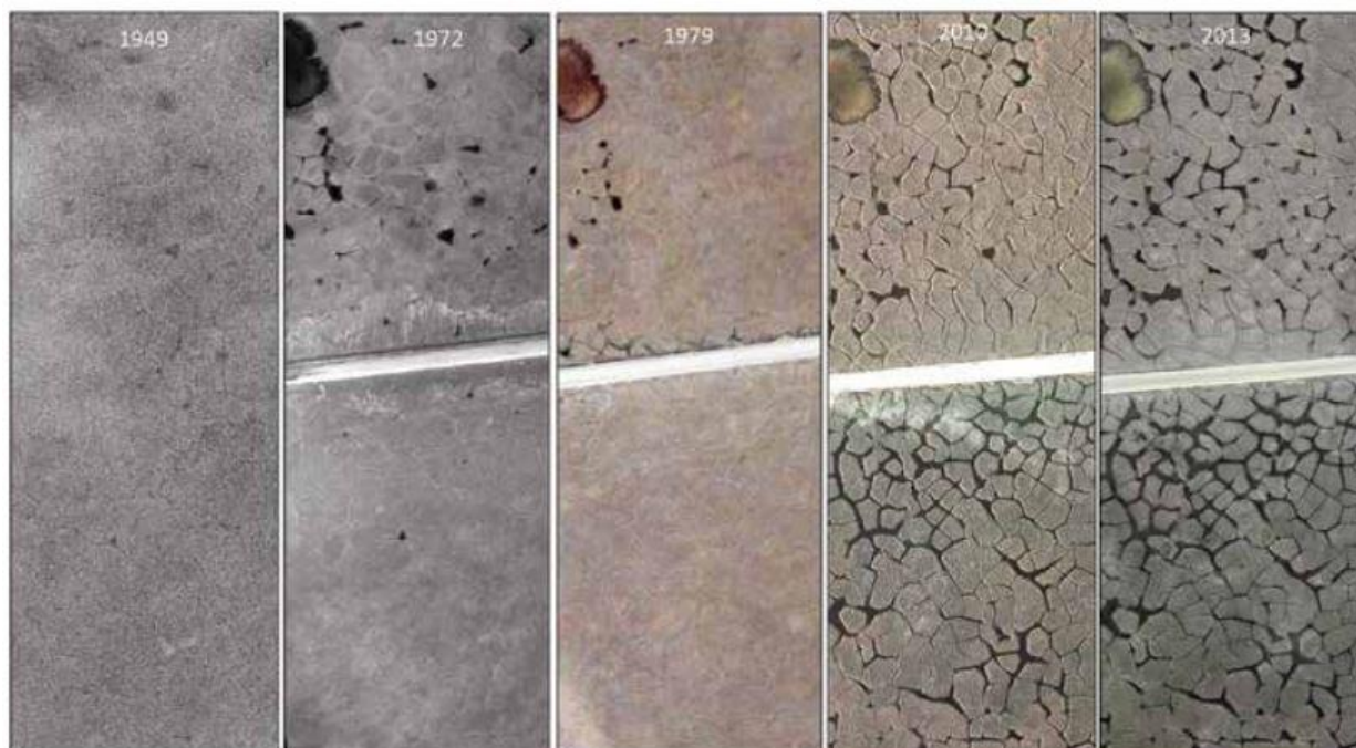
Figure 6. Adapted from Walker et al. (2014). Development of extensive thermokarst after construction of a gravel road. Aerial imagery near Lake Colleen, 1.9 mi (3 km) north of Deadhorse, Alaska.
